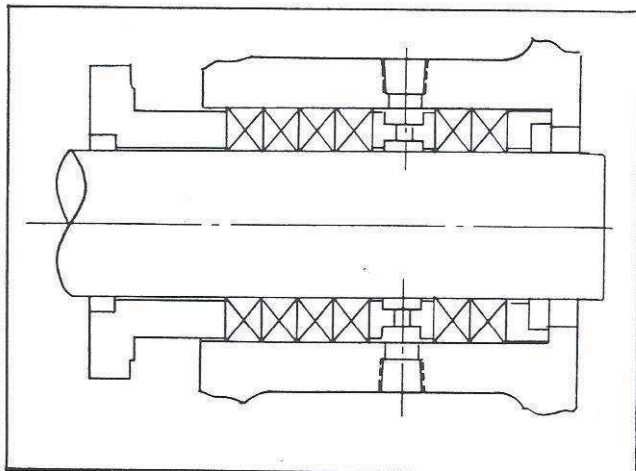
Cross section of stuffing box
