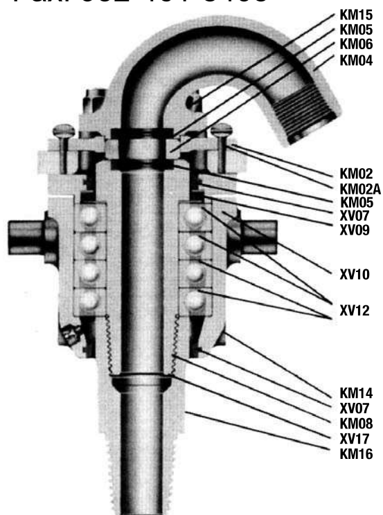
Parts List for Type 10KM Swivel
