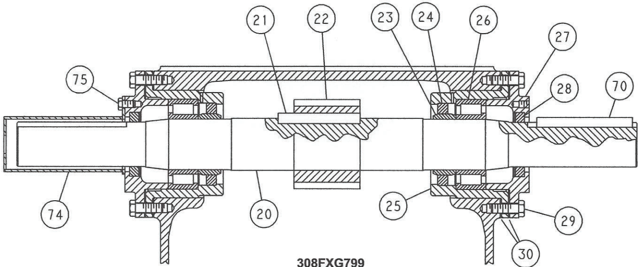
308FXG799 (Ref. Drawing)
