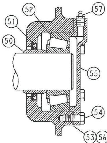
311FXG799 (Ref. Drawing)
