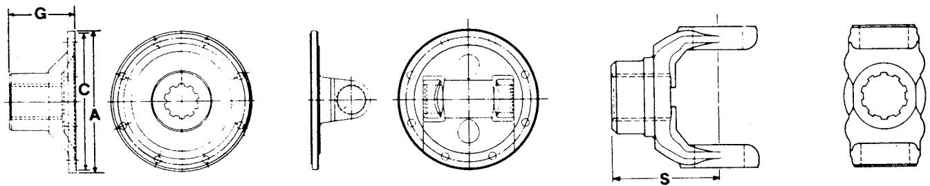
COMPANION FLANGE
